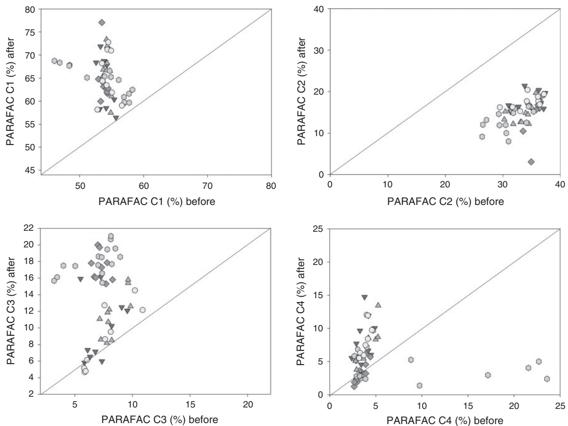
Fig. 7. Percentage of total dissolved organic matter (DOM) fluorescence associated with each parallel factor analysis (PARAFAC) component before and after 30-day incubations to measure bioavailability of dissolved organic matter (BDOC) under sunlight-exposed conditions. On each plot, a line indicates a 1 : 1 relationship. Points falling above the 1 : 1 line showed an increase in the percentage of total fluorescence associated with a particular component and points below the line indicate that a decrease was observed. Marker shape and colour indicate date of sample collection: November of 2009 (white circles), December of 2009 (dark grey inverted triangles), January of 2010 (light grey triangles), February of 2010 (grey diamonds), March of 2010 (light grey octagons), May, June, July of 2010 (dark grey squares), August of 2010 (black circles), October of 2010 (inverted black triangles).
