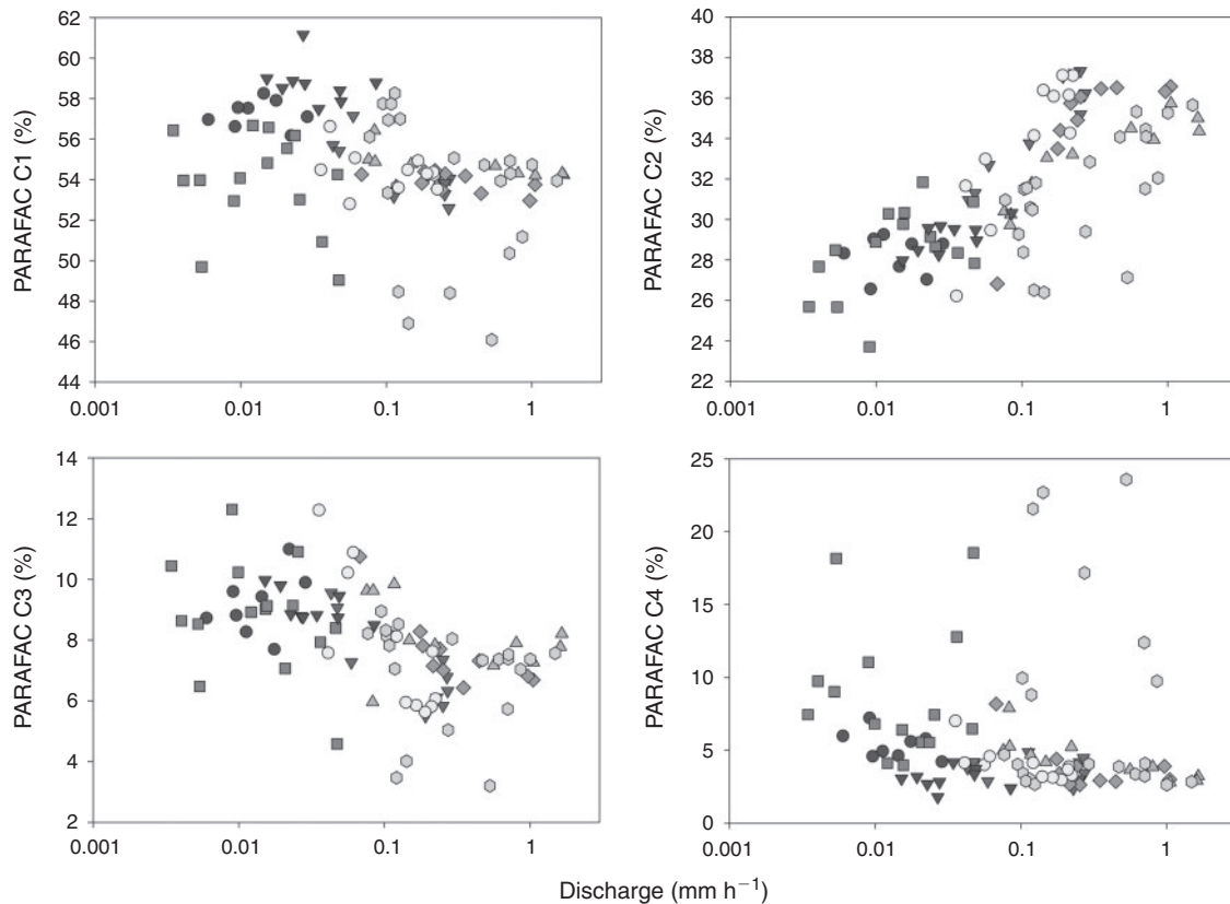
Fig. 1. The relationship between the proportion of total fluorescence associated with each parallel factor analysis (PARAFAC) component as related to discharge rate of the Upper Bigelow Brook. Marker shape and colour indicate date of sample collection: November of 2009 (white circles), December of 2009 (dark grey inverted triangles), January of 2010 (light grey triangles), February of 2010 (grey diamonds), March of 2010 (light grey octagons), May, June, July of 2010 (dark grey squares), August of 2010 (black circles), October of 2010 (inverted black triangles).
