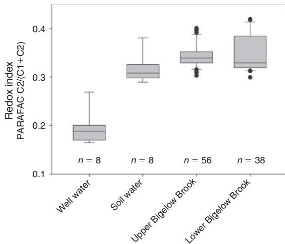
Fig. 3. Redox index of dissolved organic matter (DOM) in groundwater, soil water, and stream water of the Bigelow Brook watershed. Box plots show median, 25th and 75th percentile. Whiskers indicate the 10th and 90th percentiles. Outliers falling outside these bounds are indicated by black circles.
