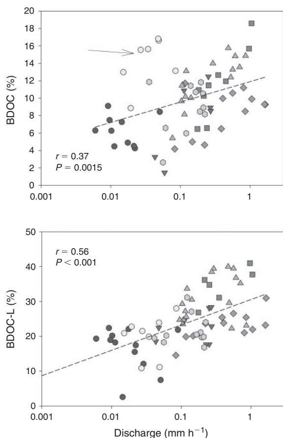
Fig. 5. Bioavailability of dissolved organic matter (BDOC) as related to discharge rate of the Upper Bigelow Brook. BDOC was measured by change in concentration over a 30-day incubation with dark (BDOC) or sunlight-exposed (BDOC-L) conditions. Marker shape and colour indicate date of sample collection: November of 2009 (white circles), December of 2009 (dark grey inverted triangles), January of 2010 (light grey triangles), February of 2010 (grey diamonds), March of 2010 (light grey octagons), May, June, July of 2010 (dark grey squares), August of 2010 (black circles), October of 2010 (inverted black triangles). An arrow points to a group of samples collected in March of 2010, with higher than expected BDOC and high tyrosine-like fluorescence ( >7\% total fluorescence).
