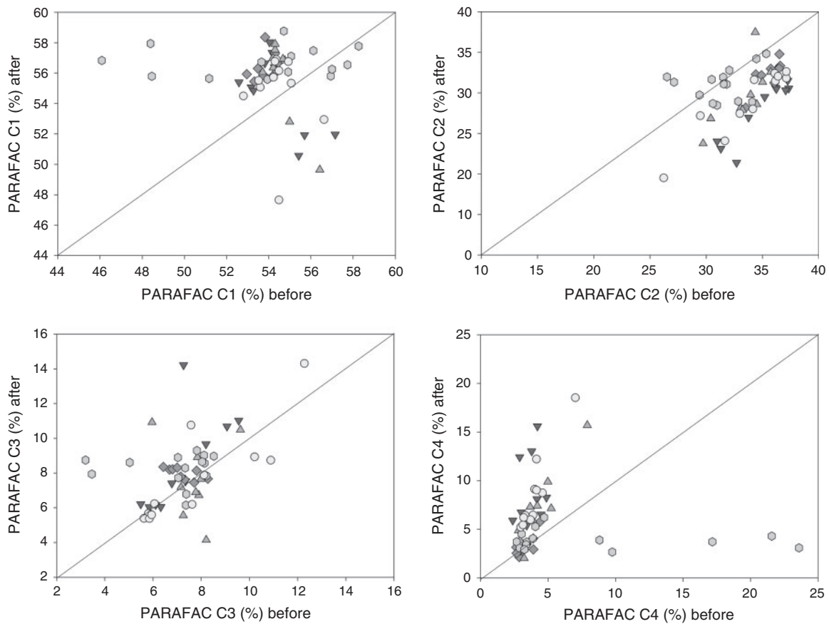
Fig. 6. Percentage of total dissolved organic matter (DOM) fluorescence associated with each parallel factor analysis (PARAFAC) component before and after 30-day incubations to measure bioavailability of dissolved organic matter (BDOC) under dark conditions. On each plot, a line indicates a 1 : 1 relationship. Points falling above the 1 : 1 line showed an increase in the percentage of total fluorescence associated with a particular component and points below the line indicate that a decrease was observed. Marker shape and colour indicate date of sample collection: November of 2009 (white circles), December of 2009 (dark grey inverted triangles), January of 2010 (light grey triangles), February of 2010 (grey diamonds), March of 2010 (light grey octagons), May, June, July of 2010 (dark grey squares), August of 2010 (black circles), October of 2010 (inverted black triangles).
