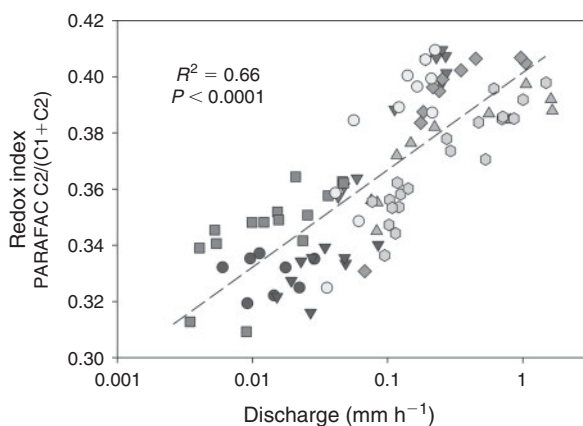
Fig. 2. Redox index of dissolved organic matter (DOM) as related to discharge rate of the Upper Bigelow Brook. Marker shape and colour indicate date of sample collection: November of 2009 (white circles), December of 2009 (dark grey inverted triangles), January of 2010 (light grey triangles), February of 2010 (grey diamonds), March of 2010 (light grey octagons), May, June, July of 2010 (dark grey squares), August of 2010 (black circles), October of 2010 (inverted black triangles).
