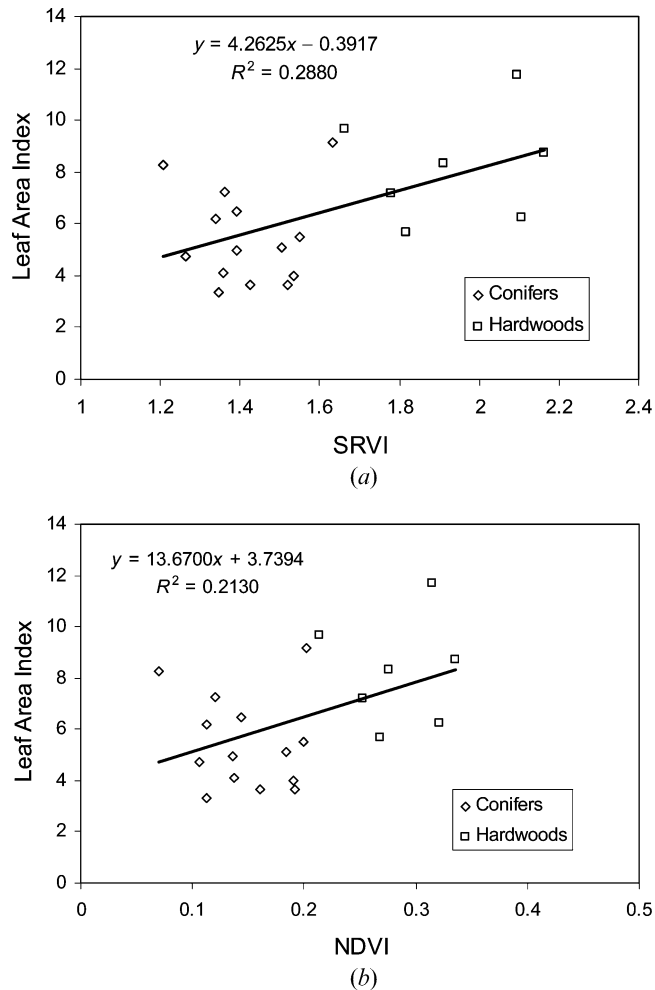
Figure 3. Relationships between spectral vegetation indices and LAI: (a) SRVI and (b) NDVI. Diamonds ( \diamond ) indicate conifer and squares ( \square ) indicate hardwood dominated stands.
