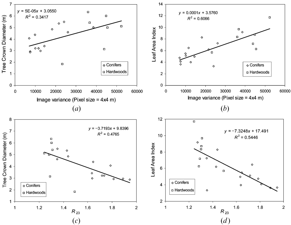
Figure 2. Relationships between image spatial information and canopy structural parameters for pooled conifer and hardwood stands: (a) tree crown size versus image variance at 4 × 4 m spatial resolution, (b) LAI versus image variance at 4 × 4 m spatial resolution, (c) tree crown size versus ratio of image variances at 2 × 2 to 3 × 3 m spatial resolutions and (d) LAI versus ratio of image variances at 2 × 2 to 3 × 3 m spatial resolutions.
