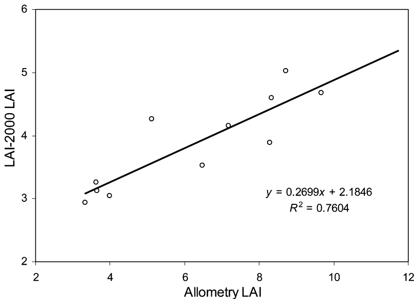
Figure 1. The relationship between effective LAI measured by LAI-2000 and LAI estimated from allometry. The strong relationship indicates that the LAI estimated from allometry is consistent among stands.
