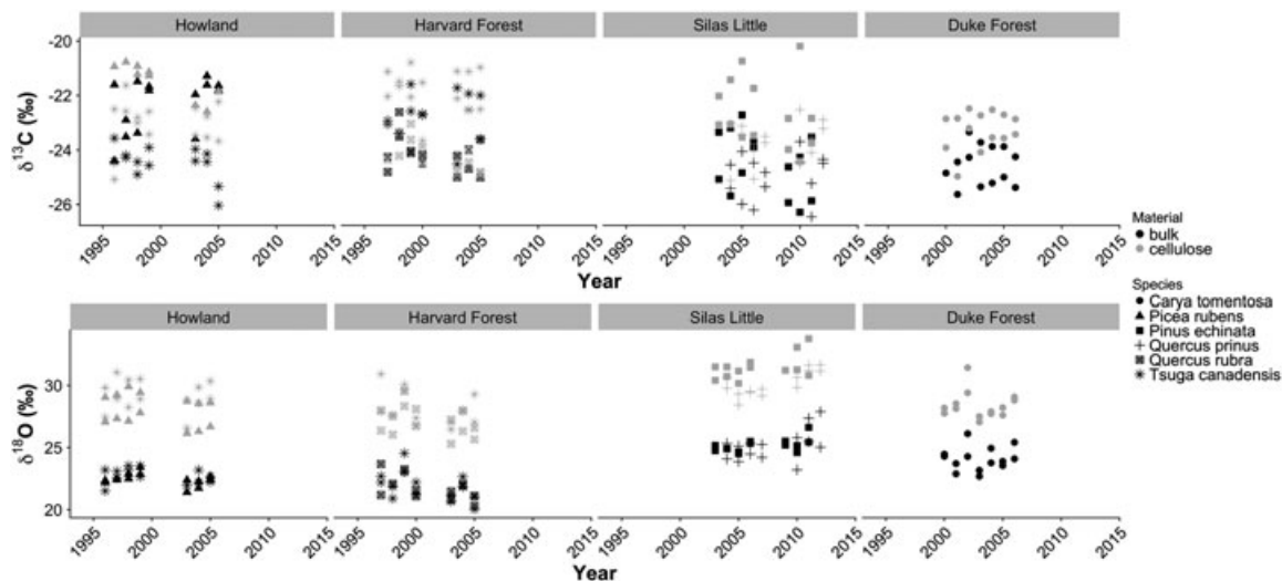
FIGURE 1 \delta^{13}\text{C} and \delta^{18}\text{O} values measured for each species ( n = 2 trees per species) across the seven selected years of study. Sites in the panels are arranged according to their latitude (from 45^{\circ}20'\text{N} to 35^{\circ}9'\text{N} ). The dry years for each site: 1999 for Howland, 1997 for Harvard Forest, 2005 and 2010 for Silas Little and 2002 and 2005 for Duke Forest
