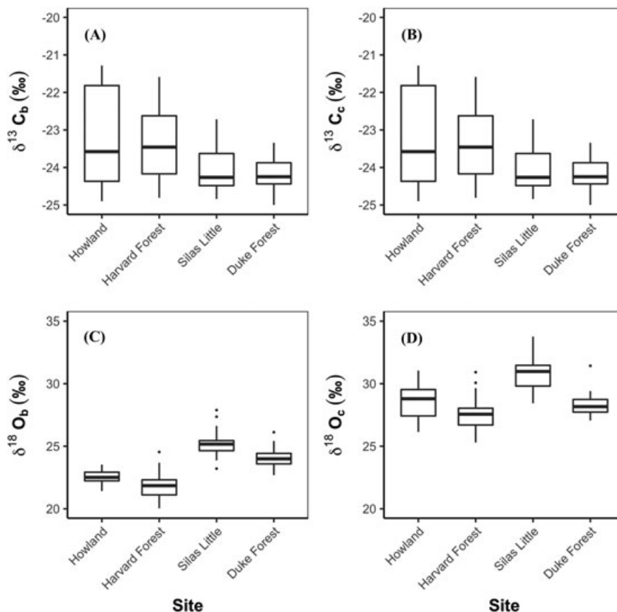
FIGURE 2 Boxplots showing \delta^{13}\text{C} and \delta^{18}\text{O} values measured in bulk ( \delta^{13}\text{C}_b and \delta^{18}\text{O}_b ) (A, C) and \alpha -cellulose ( \delta^{13}\text{C}_c and \delta^{18}\text{O}_c ) (B, D) for the two dominant species at the four investigated AmeriFlux sites. Sites in the x-axis are arranged according to their latitude (from 45^\circ 20' to 35^\circ 97'N )
