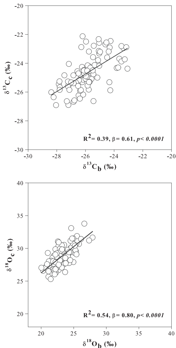
FIGURE 3 Relationship between bulk wood and \alpha -cellulose for \delta^{13}\text{C} (top) and \delta^{18}\text{O} values (bottom)
