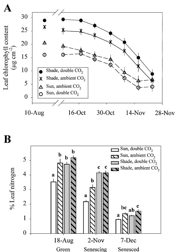
Fig. 4 (a) Chlorophyll content throughout the course of autumnal senescence ( N=12 ); symbols are the same as in Figs 2 and 3. Measurements in August prior to the onset of senescence are shown before the break in the x-axis. (b) Nitrogen concentration of leaves ( \text{g N } [100 \text{ g leaf}]^{-1} ), measured in August before the onset of senescence, during senescence, and after all leaves had turned brown. Leaves had completely senesced by December. Treatments are shown as different if P < 0.05 (Scheffé's posthoc multiple comparisons). Error bars are \pm 1 SE.
