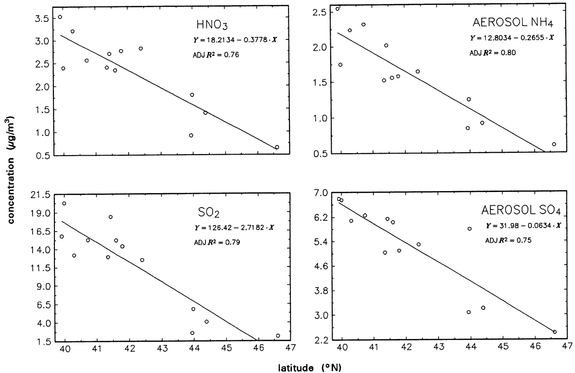
FIG. 5. Regression plots of mean annual air concentrations of dry-deposited species against latitude. Note that longitude is also a significant predictor for \text{SO}_2 and aerosol \text{SO}_4^{2-} (Table 2). No trend was observed for aerosol \text{NO}_3^- so its regional mean value ( 0.75 \mu\text{g}/\text{m}^3 ) was used for all locations.
