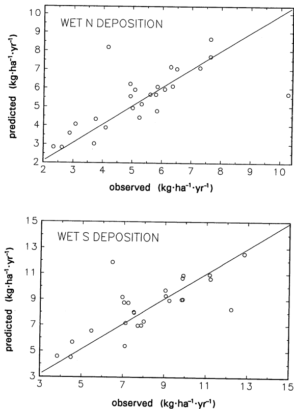
FIG. 4. Plots of predicted vs. observed wet deposition of nitrogen (from \text{NO}_3^- + \text{NH}_4^+ ) and sulfur at the 26 NADP/NTN collection stations used in this study.
