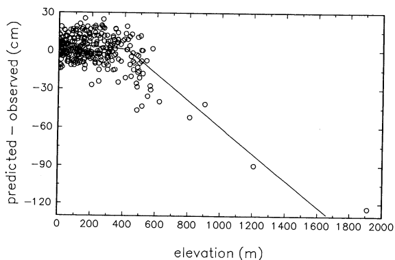
FIG. 3. Variation of annual precipitation with elevation, as shown by plotting residuals vs. elevation from a regression of mean annual precipitation against latitude and longitude (residuals = predicted - observed values, n = 310 ). The line represents the elevation effect described by a dummy variable regression indicating a significant discontinuity at \approx 400 m.
