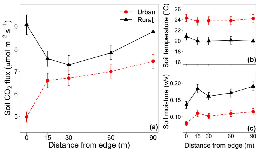
FIGURE 2 Mean soil respiration rates ( \mu\text{mol CO}_2 \text{ m}^{-2}\text{s}^{-1} ) as a function of distance from the edge (a) for urban and rural sites during the mid-growing season (June 1–September 15). Mean mid-season soil temperature (b; ^\circ\text{C} ) and volumetric soil moisture (c; v/v) point measurements were taken at the time of respiration measurement. Measured respiration, temperature, and moisture are data shown; bars around each point are standard error around the mean [Colour figure can be viewed at wileyonlinelibrary.com ]
