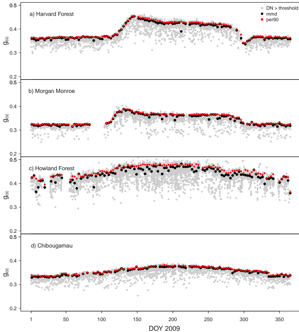
Fig. 6. Three-day green chromatic coordinate ( g_{cc} ) obtained as mean mid-day values ( mmd ) and as the 90th percentile of all day-time values within a three-day moving window ( per90 ) at two deciduous-dominated forest sites: (a) Harvard Forest and (b) Morgan Monroe State Forest, and at two coniferous-dominated forest sites: (c) Howland Forest and (d) Chibougamau (Table 1). The green chromatic coordinate was filtered for digital camera-specific RGB thresholds (digital number ( DN ) > threshold; see Table 3 and text for further explanation). (For interpretation of the references to color in this figure legend, the reader is referred to the web version of the article.)
