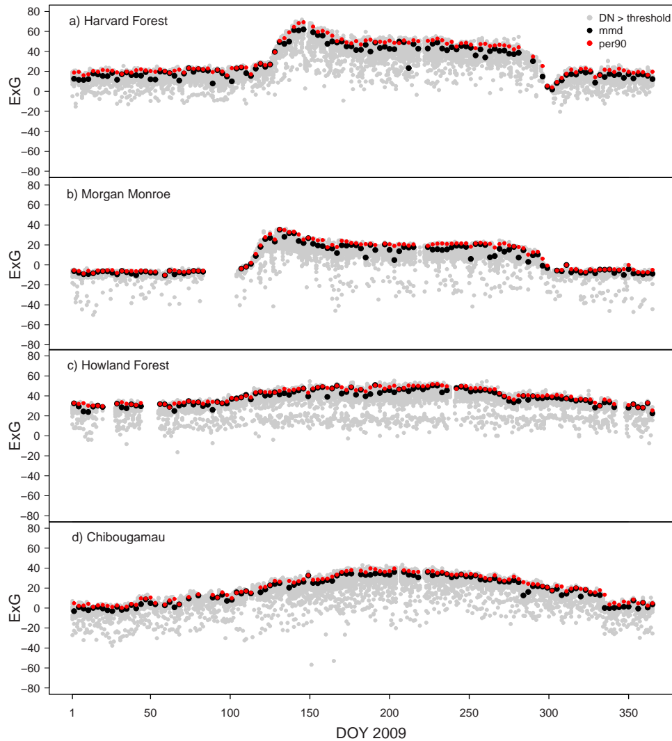
Fig. 5. Three-day green excess ( ExG ) obtained as mean mid-day values ( mmd ) and as the 90th percentile of all day-time values within a three-day moving window ( per90 ) at two deciduous-dominated forest sites: (a) Harvard Forest and (b) Morgan Monroe State Forest, and at two coniferous-dominated forest sites: (c) Howland Forest and (d) Chibougamou (Table 1). The green chromatic coordinate was filtered for digital camera-specific RGB thresholds (digital number ( DN ) > threshold; see Table 3 and text for further explanation). (For interpretation of the references to color in this figure legend, the reader is referred to the web version of the article.)
