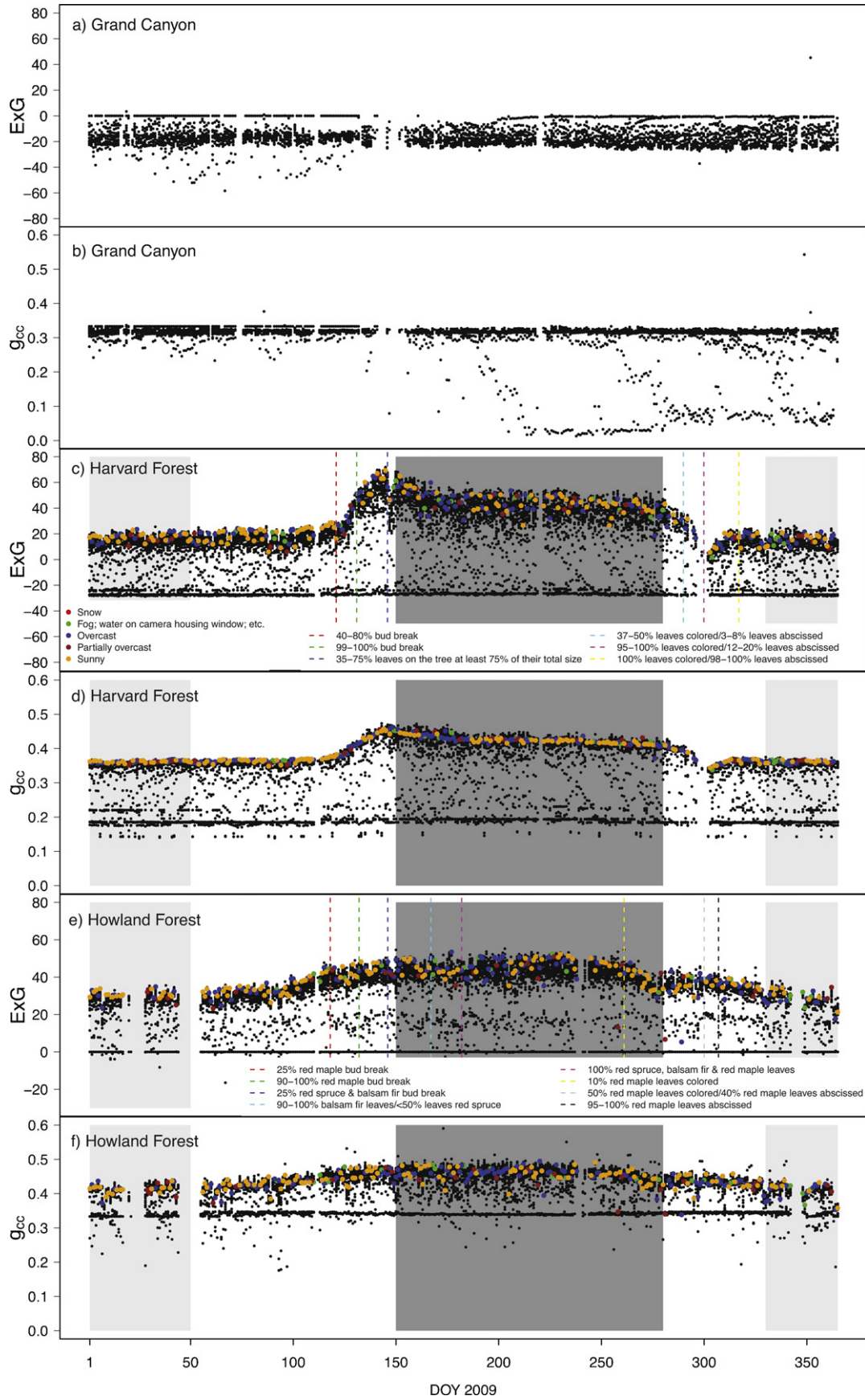
Fig. 3. Example data set of (a) excess green ( ExG ) and (b) the green chromatic coordinate ( g_{cc} ) for Grand Canyon, of (c) ExG (including observer-based estimates of spring and autumn phenology for red oak [O’Keefe, 2000]) and (d) g_{cc} for Harvard Forest, of (e) ExG (including observer-based estimates of spring and autumn phenology for red spruce, eastern hemlock, and red maple [Richardson et al., 2007]) and (f) g_{cc} for Howland Forest (red rectangle region-of-interests for the dominant tree species in Fig. 1a and b). The
