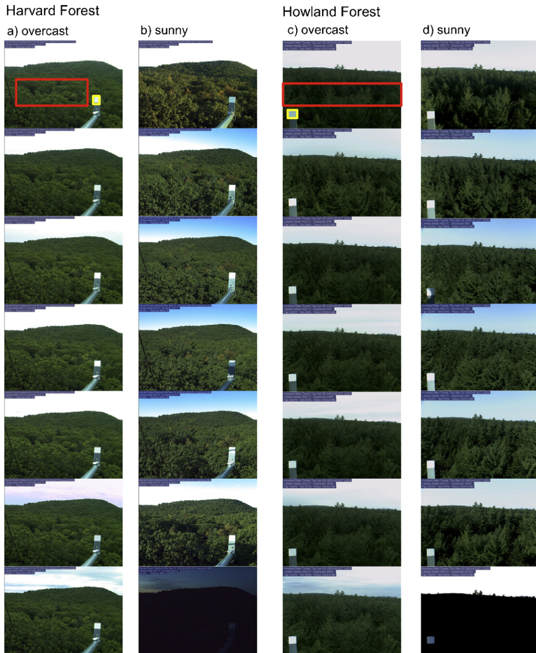
Fig. 1. Example images (from top to bottom: 06:00; 08:00; 10:00; 12:00; 14:00; 16:00; 18:00 h local time) from deciduous-dominated Harvard Forest during (a) an overcast (DOY 156) and (b) a sunny day (DOY 264), and from coniferous-dominated Howland Forest during (c) an overcast (DOY 160) and (d) a sunny (DOY 253) day from summer 2009. The red and yellow rectangles are the regions-of-interest for the dominant tree species and the reference panels, respectively. (For interpretation of the references to color in this figure legend, the reader is referred to the web version of the article.)
