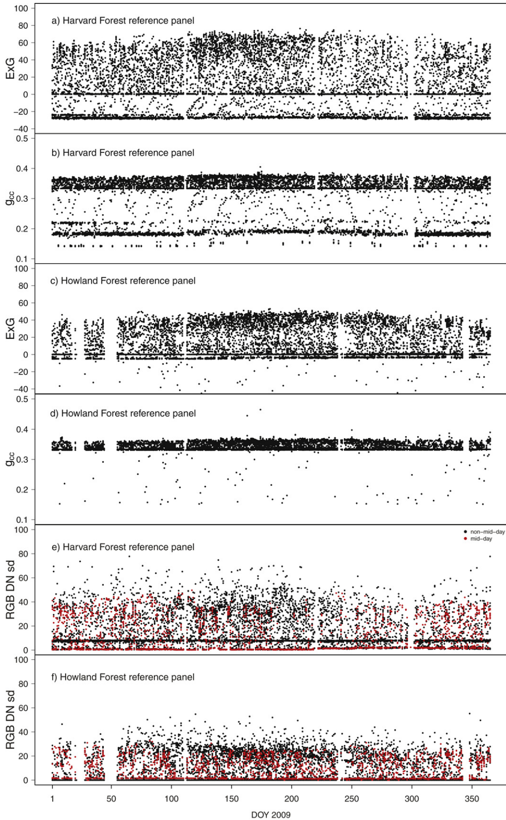
Fig. 2. Reference panel (a) excess green ( ExG ), and (b) green chromatic coordinate ( g_{cc} ) for Harvard Forest, reference panel (c) ExG , and (d) g_{cc} for Howland Forest, (e) RGB standard deviation ( sd ) for Harvard Forest (yellow rectangle region-of-interest [ROI] in Fig. 1a), and (f) RGB sd for Howland Forest (yellow rectangle ROI in Fig. 1b). Mid-day covers the period between 10:00 and 14:00 h (local time), whereas non-mid-day hours covers periods before 10:00 and after 14:00 h. (For interpretation of the references to color in this figure legend, the reader is referred to the web version of the article.)
