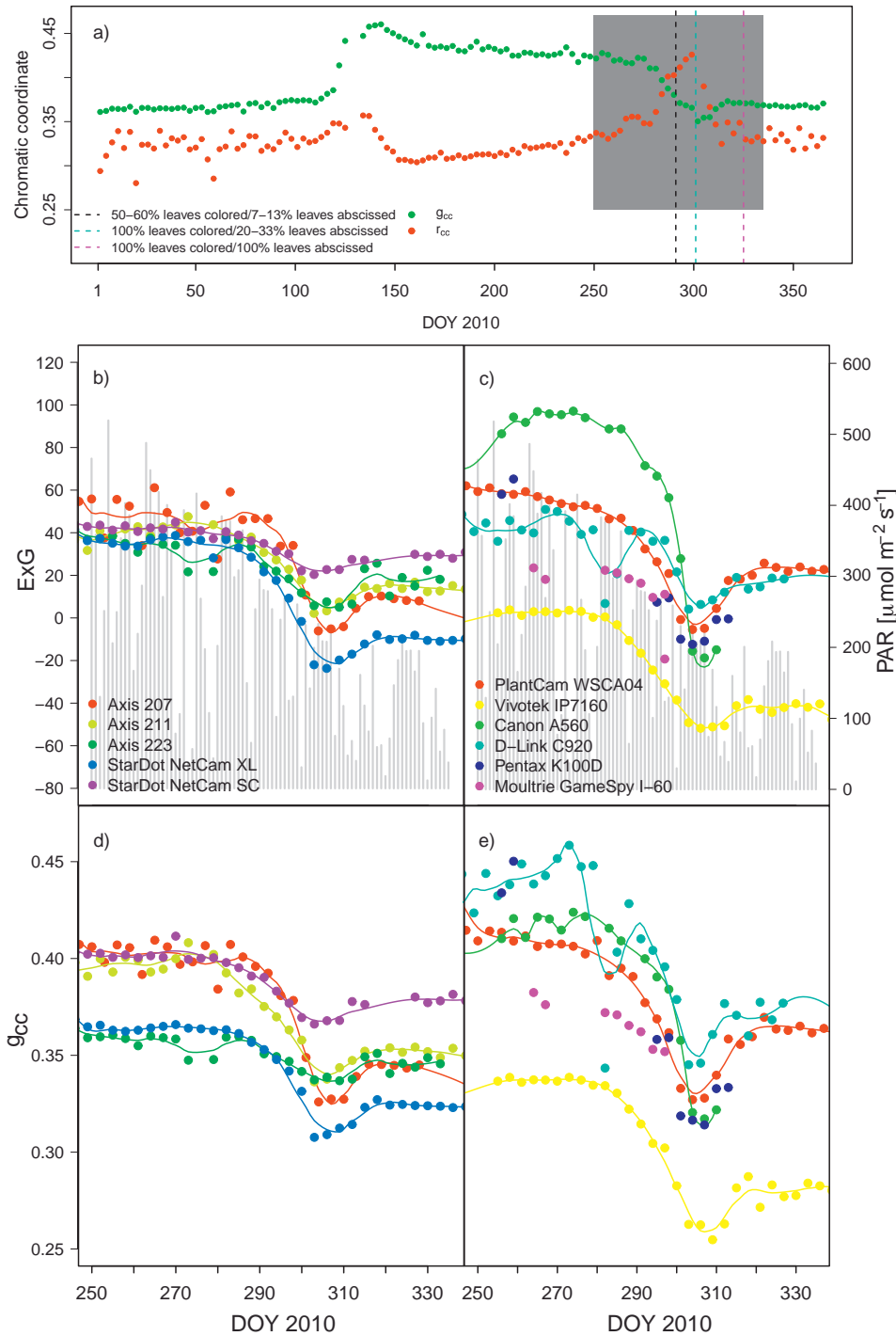
Fig. 8. Three-day (a) green ( g_{cc} ) and red ( r_{cc} ) chromatic coordinates at the deciduous-dominated Harvard Forest in 2010 (dark-grey shading indicates the observation period including observer-based estimates of red oak autumn phenology), three-day (b) and (c) excess green (ExG) and mean daily incoming photosynthetically active radiation (PAR) as grey-bar backdrop, and (d) and (e) g_{cc} calculated from RGB brightness levels obtained with eleven different digital cameras (Fig. 7) at Harvard Forest (ancillary instrumentation tower). Also included in panels (b)–(e) are daily fitted Loess-curves (span=0.30) for both ExG and g_{cc} . (For interpretation of the references to color in this figure legend, the reader is referred to the web version of the article.)
