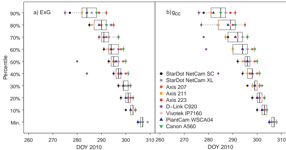
Fig. 9. Comparison of between-digital camera variation in day-of-year (DOY) for complete leaf coloring (i.e., minimum [Min.] canopy greenness) and for different percentiles (10th–90th) of daily Loess curves (span=0.30) fitted to three-day (a) excess green ( ExG ) and (b) the green chromatic coordinate ( g cc ) obtained as the 90th percentile of all day-time values within a three-day moving window ( per90 ). We excluded the Moultrie Game Spy I-60 and the Pentax K100D due to large gaps caused by battery leakage and failure, respectively. (For interpretation of the references to color in this figure legend, the reader is referred to the web version of the article.)
