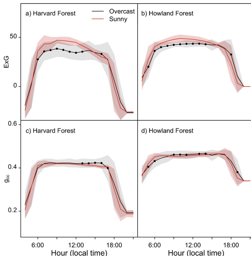
Fig. 4. Mean diurnal patterns ( \pm one standard deviation [shaded areas]) of excess green ( ExG ) at (a) Harvard Forest and at (b) Howland Forest, and of the green chromatic coordinate ( g_{cc} ) at (c) Harvard Forest and at (d) Howland Forest for overcast and sunny days (see text for further explanation) over the summer period in 2009 (dark-grey shading in Fig. 2). The black dots indicate significant differences between the overcast and sunny conditions (Wilcoxon signed-rank test; p < 0.05 ). (For interpretation of the references to color in this figure legend, the reader is referred to the web version of the article.)
