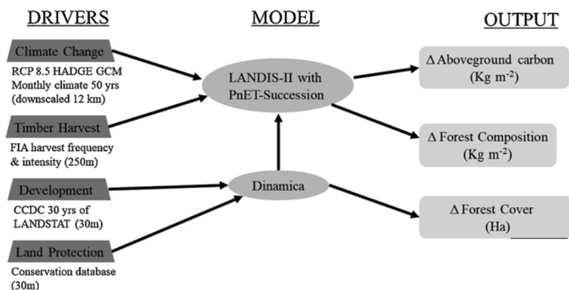
Fig. 2. Conceptual framework illustrating our simulation approach. The diagram represents some of the multiple drivers of land-use change including data sources and spatial resolution. Additional model variables are described in methods. The drivers are spatial variables in the models which affect the outputs.
