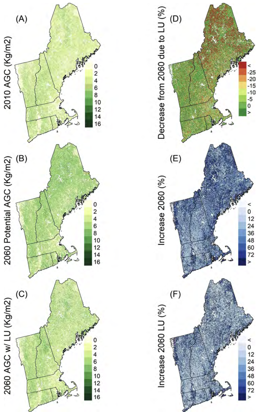
Fig. 4. New England maps of: (A) AGC at year 2010; (B) AGC at year 2060 without land use; (C) AGC at year 2060 with land use; (D) percent change in AGC with land use at year 2060 from year 2060 without land use; (E) percent change in AGC without land use at year 2060 from year 2010; (F) percent change in AGC with land use at year 2060 from year 2010. All 2060 map results include climate change.
